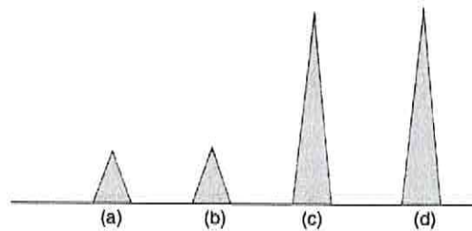
Fig. 3. Two minor alleles, a and b , with two major alleles, c and d , where allele b is in a stutter position.
