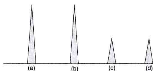
Fig. 1. A four-allele mixture, showing major ab and minor cd contributions.
