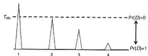
Fig. 6. Alleles 1–4 are phenotypic homozygotes of decreasing size. The probability of drop-out \Pr(D) increases as the size of the surviving peak decreases.
