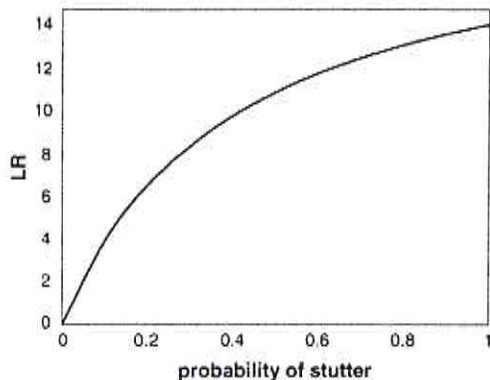
Fig. 5. Plot of \Pr(\text{St}) vs. 1/(p_a^2 + 2p_a p_c + 2p_a p_d + (2p_a p_b/\Pr(\text{St}))) , where p_a = p_b = p_c = p_d = 0.1 . The suspect is a minor contributor aa , the victim is (major) cd and allele b is present at the stutter position.
