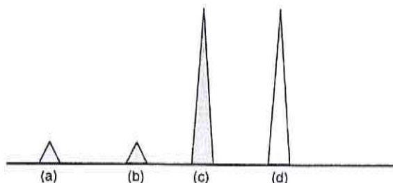
Fig. 4. c and d are unambiguous alleles, b is a minor allele in a stutter position and a is an unambiguous minor allele.
