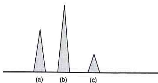
Fig. 2. A three-allele profile showing masking.
